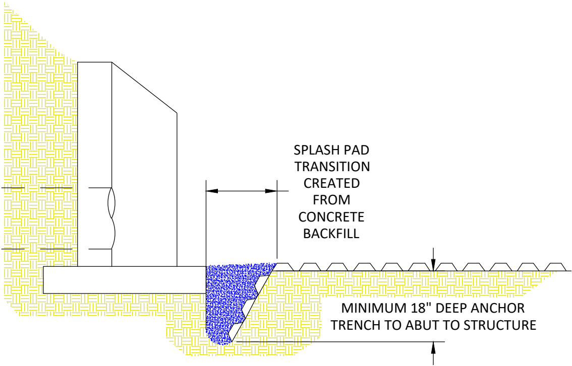
PROFILE VIEW OF ANCHOR TRENCHES
