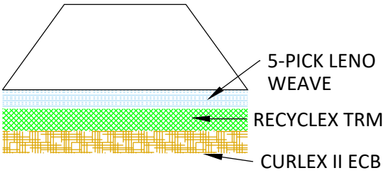
FLEXAMAT PLUS UNDERLAYMENT
