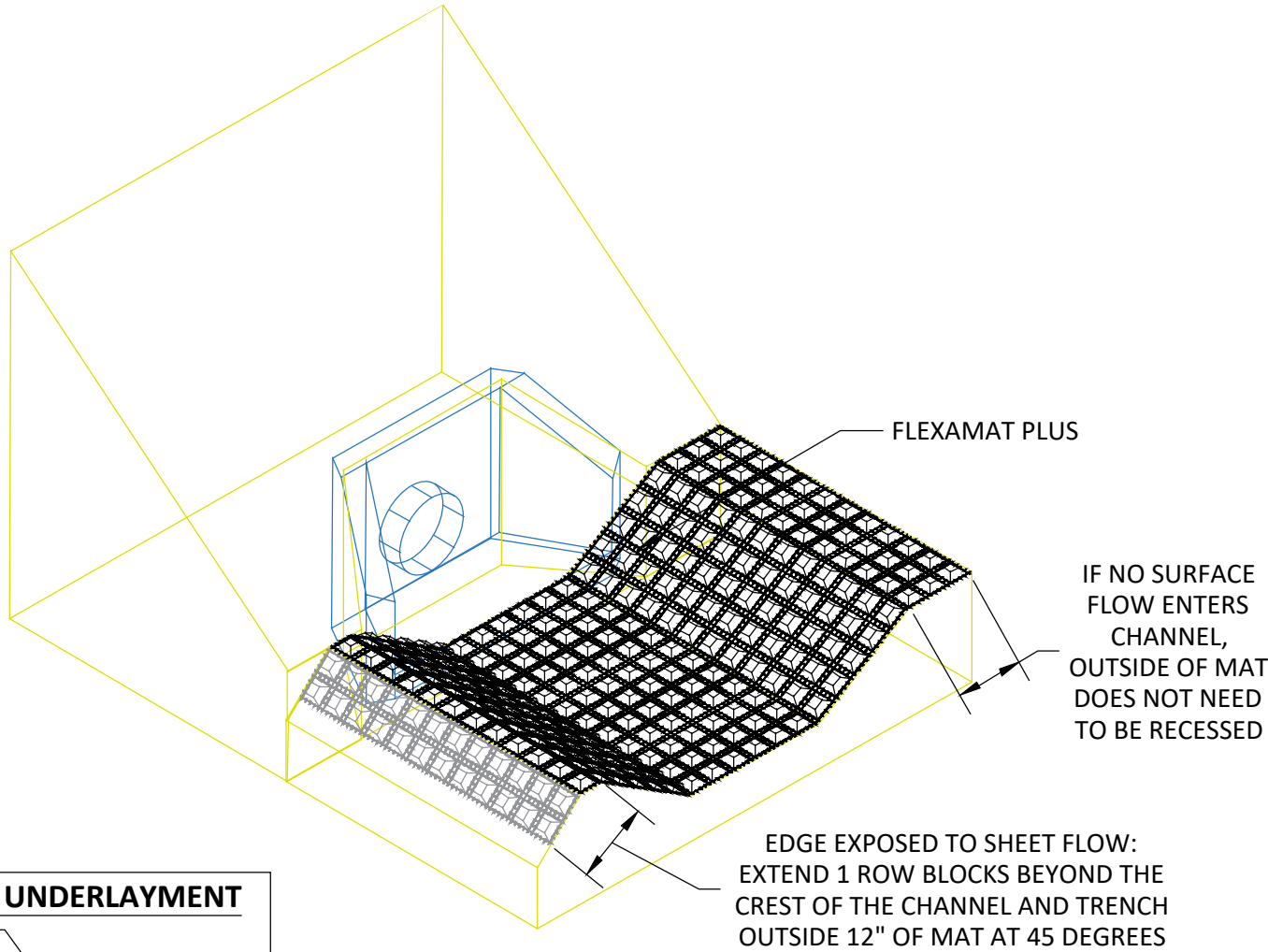
ISOMETRIC VIEW OF OUTLET AND SLOPE PROTECTION
